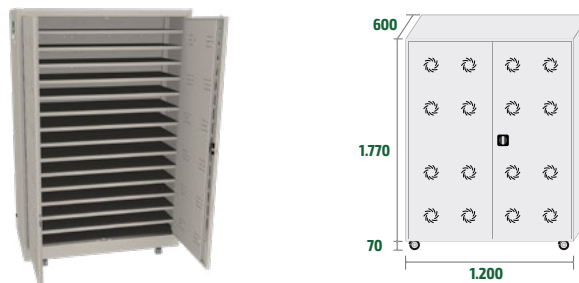
CHARGING CART 60P 60 PORTÁTILES
