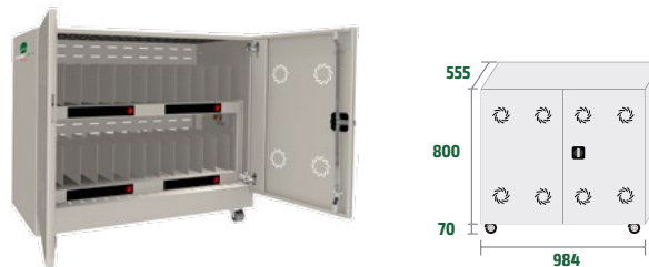
CHARGING CART 24P ECO 24 PORTÁTILES
